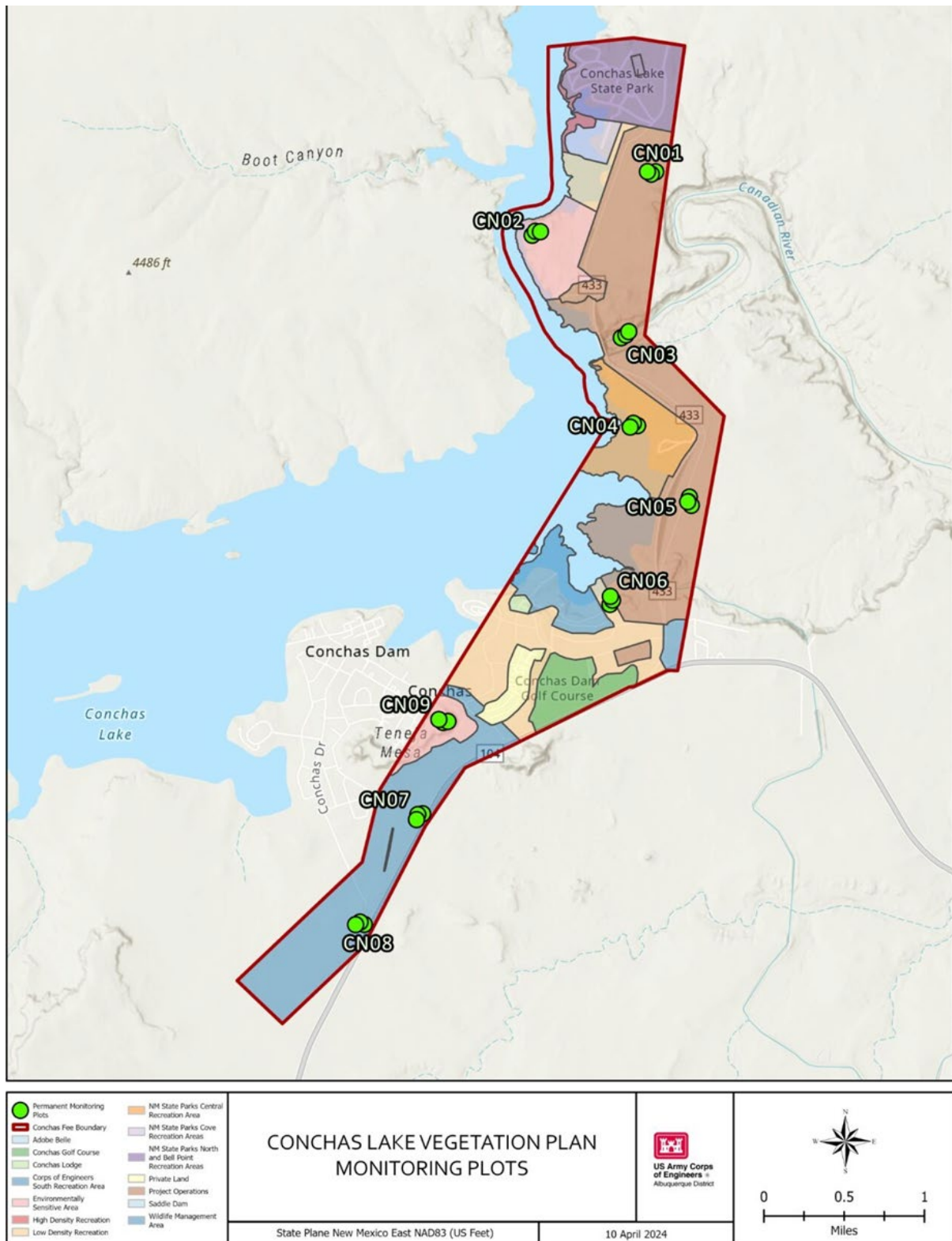
Figure 17: Permanent Monitoring Plot locations overlayed on Land Use Classifications within Conchas Dam Fee Boundary.
